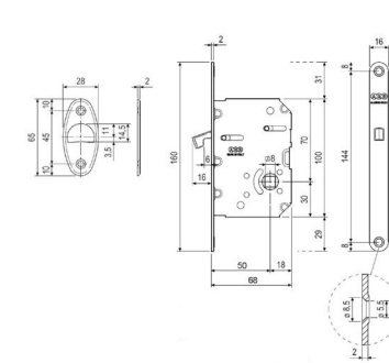
SD226 set rosette incasso con nottolino q.8 mm con frontale + serratura sliding door handle set with turn and release 8 mm square spindle with flush pull hole + lock
