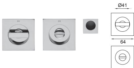
SD224 set rosette incasso con nottolino q. 8 mm con frontale sliding door handle set with turn and release 8 mm square spindle and flush pull hole
