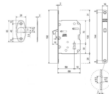
2194/SE108 set rosette incasso con nottolino q.8 mm con frontale + serratura sliding door handle set with turn and release 8 mm square spindle with flush pull hole + lock
